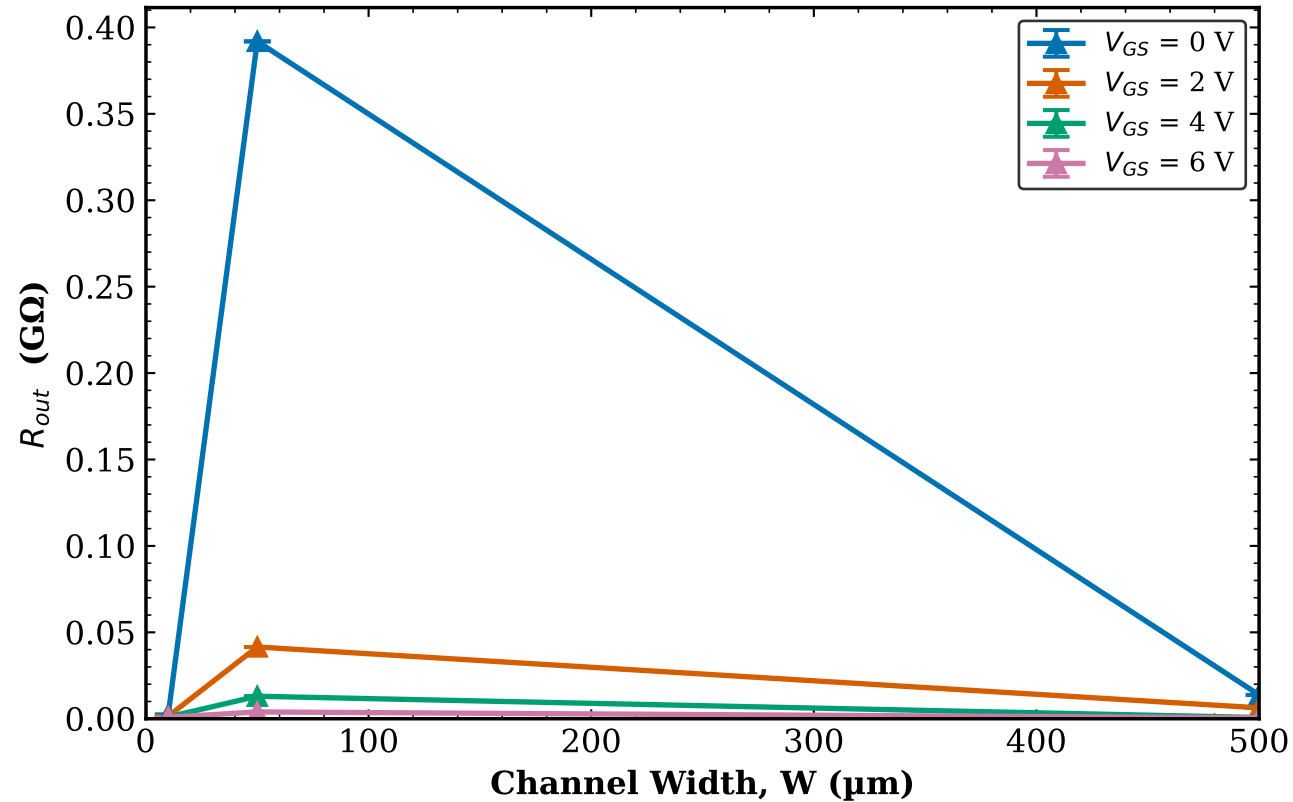
TFT2 Transistor 1 R_{out} vs W | L = 40\text{ }\mu\text{m}
